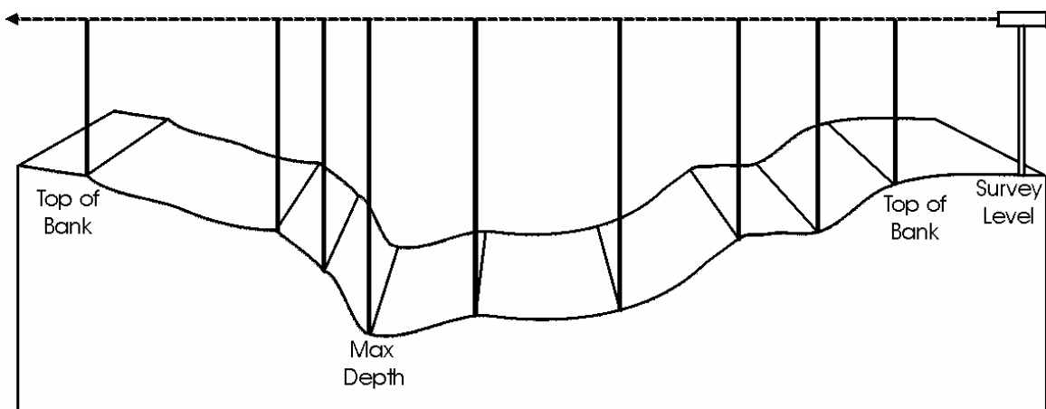
Figure 5: Survey all major slope changes across the active channel.
