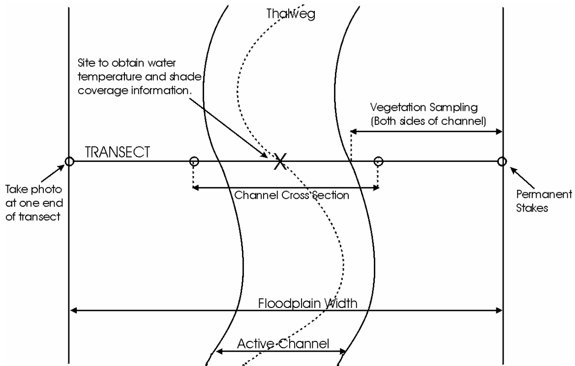
Figure 4: Transect setup for monitoring surveys.
