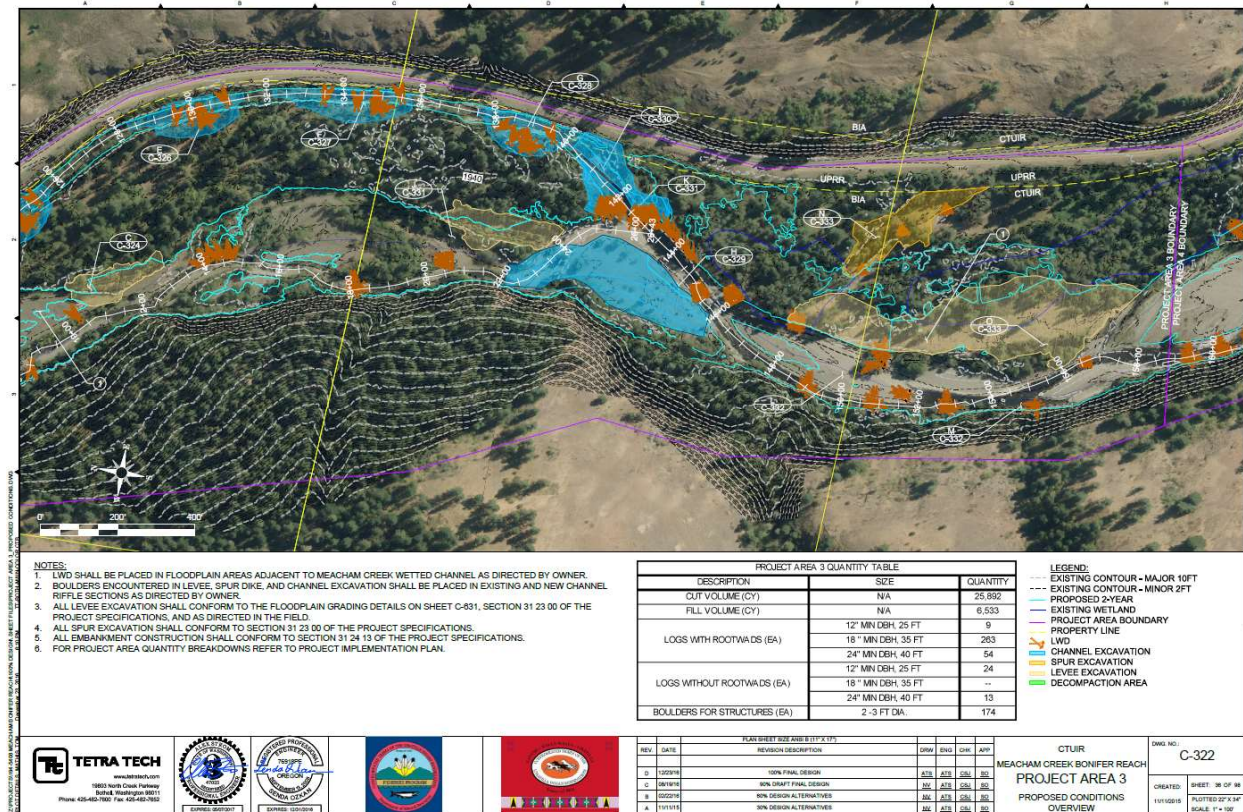
Figure 9. Meacham Creek – Bonifer Floodplain Restoration Project Example Final Design Features, RM 1.9-5.7.
