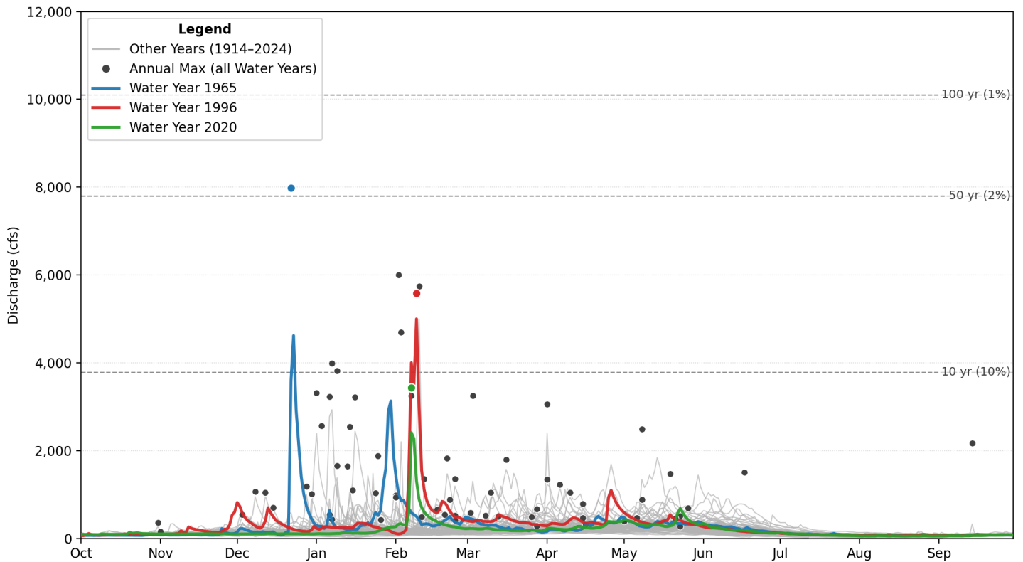
Tucannon at Starbuck (USGS-13344500) Daily Hydrographs by Water Year (Oct-Sep)
